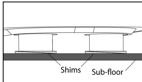
FIGURE 3. Shim feet if needed using construction adhesive to attach shims to bathtub feet and subfloor.
