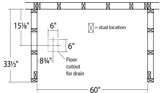
6032 Stud Layout. Keating™ Seated Base Designed for use with 32" x 60" bathtub walls
